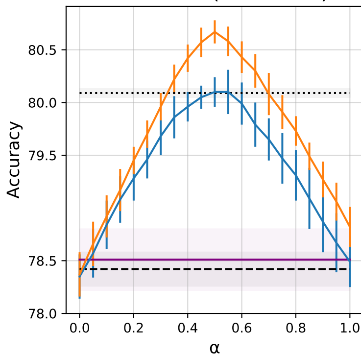
CIFAR100 (ResNet18)
